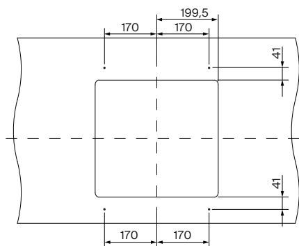
KBK 110-40
