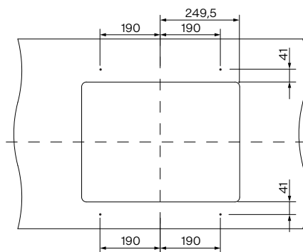
KBK 110-50 / KBK 160
