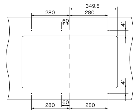
KBK 110-70
